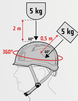
IMPACT TEST
