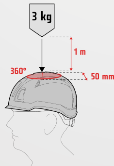
PENETRATION TEST
