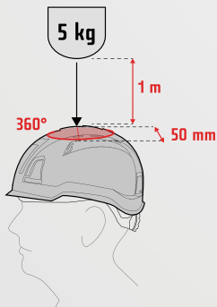
IMPACT TEST
