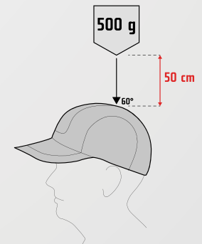
PENETRATION TEST
