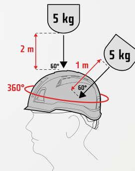
IMPACT TEST
