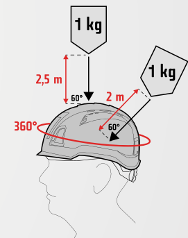
PENETRATION TEST
