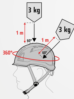
PENETRATION TEST
